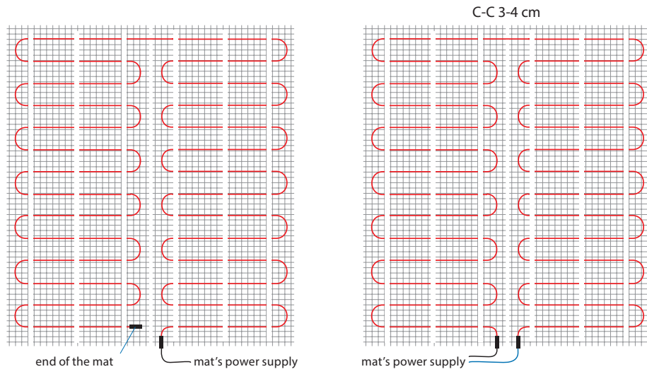
Fig. 7. Example of layout of a single conductor heating mat.
