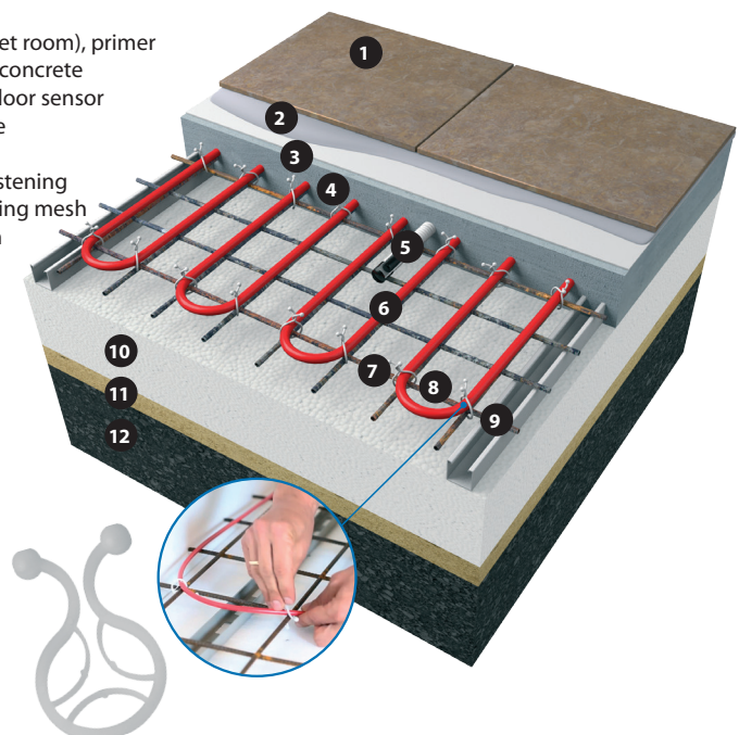
Fig. 5. Cable heating in concrete with cable fixed to reinforcement mesh by DEViClip™ Twist.
