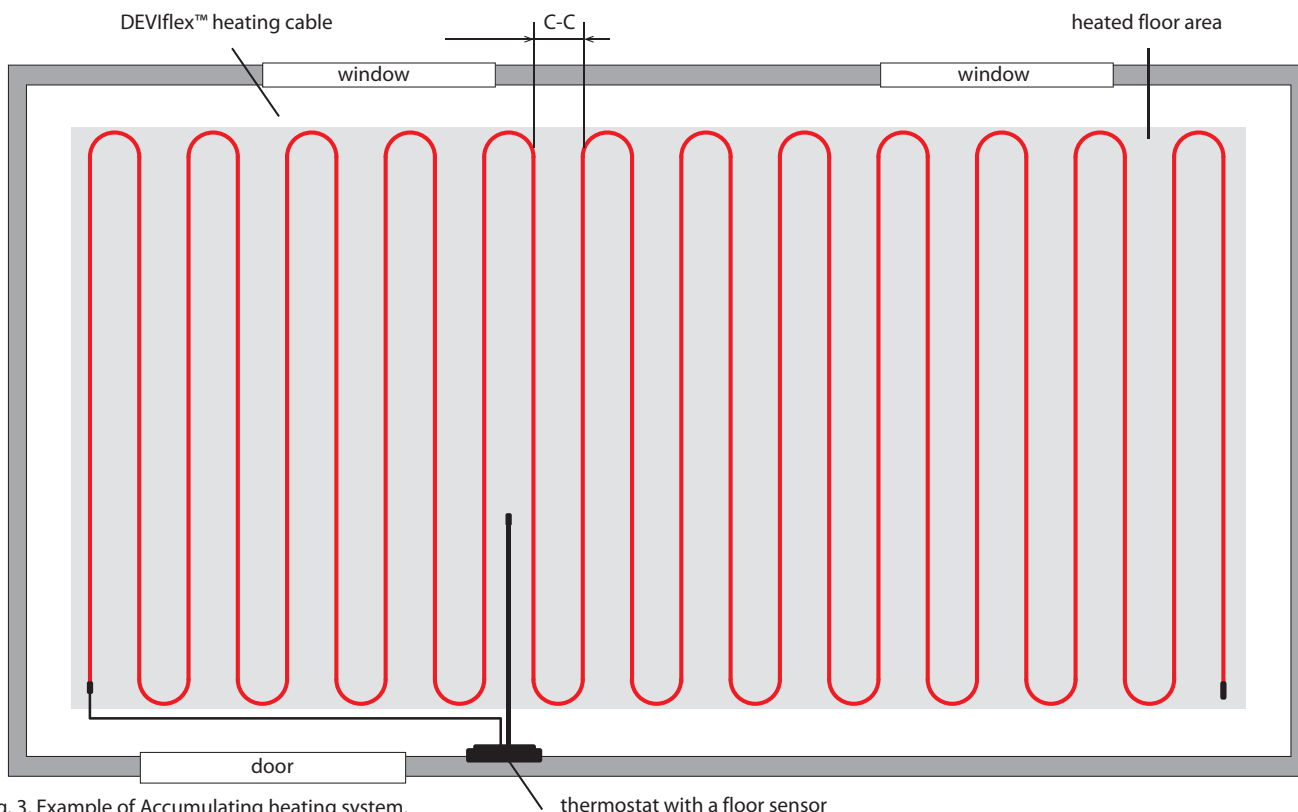
Fig. 3. Example of Accumulating heating system.
