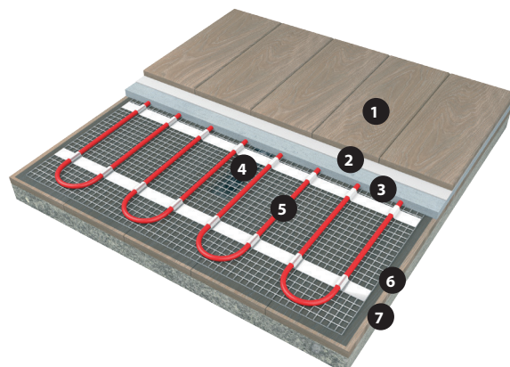
Fig. 12 – Wooden floor on thin floor
