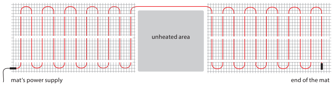
Fig. 8. Layout for a mat around an unheated area / obstacle.
