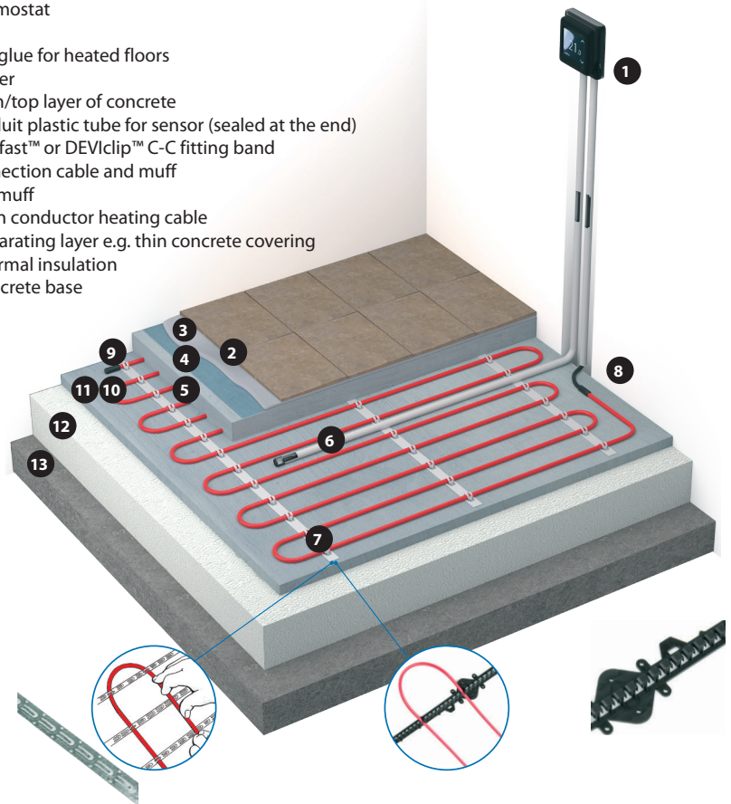
Fig. 4. Cable heating in concrete floor with cable fixed by DEVIfast™ or DEViClip™ C-C fitting band.
