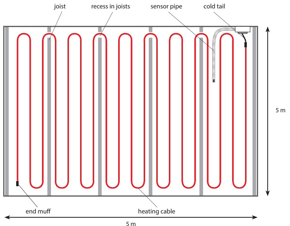
Fig. 14. Wooden floor on joists
