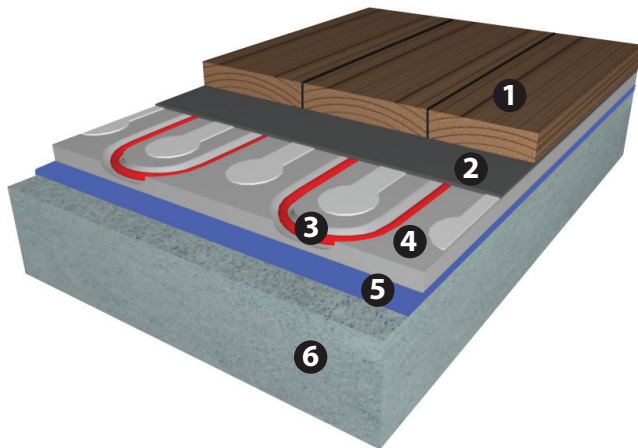
Fig. 21. Floor heating with DEVIcell™ on concrete floors
