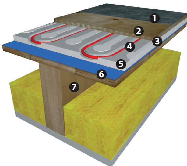
Fig. 22. Floor heating with DEVIcell™ on existing wooden floors
