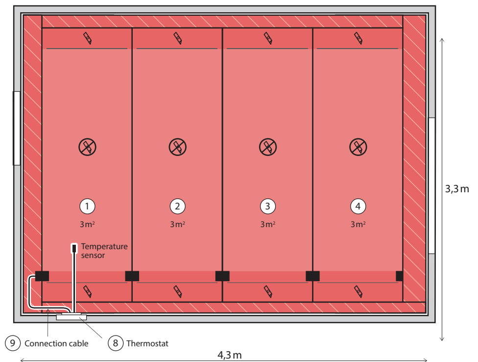
Fig. 19. Connectors along bottom wall and place for thermostat installation is bottom-left corner of the room.
