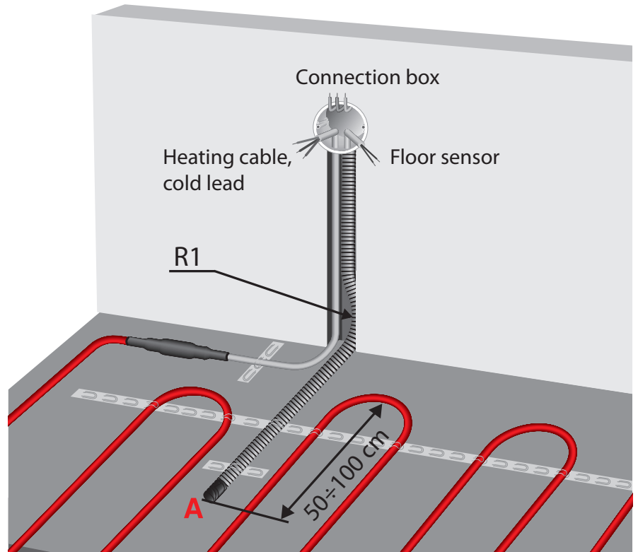
Sensor has to be installed between two heating cables and, preferably, slightly above their level.
