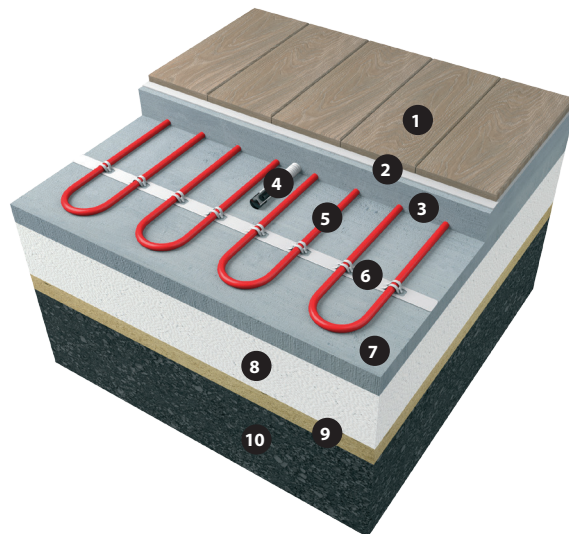
Fig. 11 – Wooden floor on concrete
