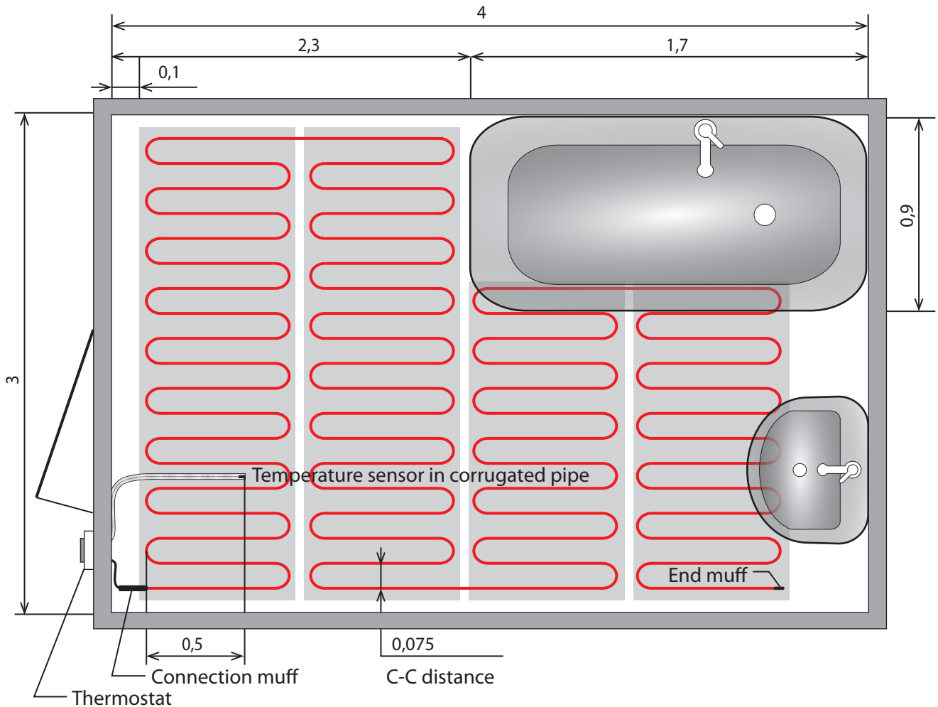
Figure 1 – Example of heating mat installation in bathroom. All distances are in [m].
