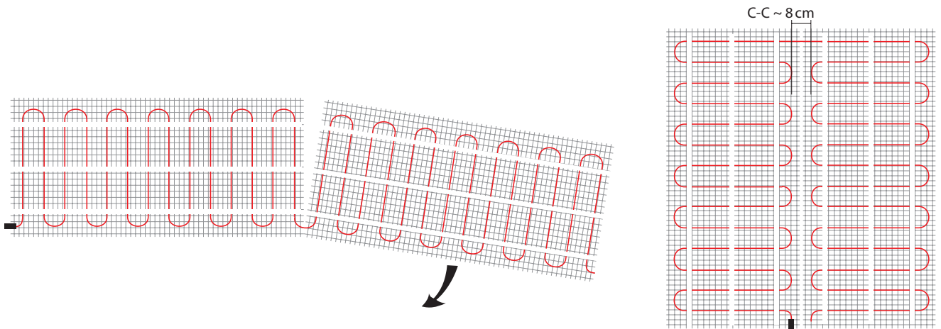
Fig. 9. The heating mats can be very easily adapted to the shape of the heated surface. Example above: placing DEVImat™ 150T 50 x 300 cm on 100 x 150 cm.
