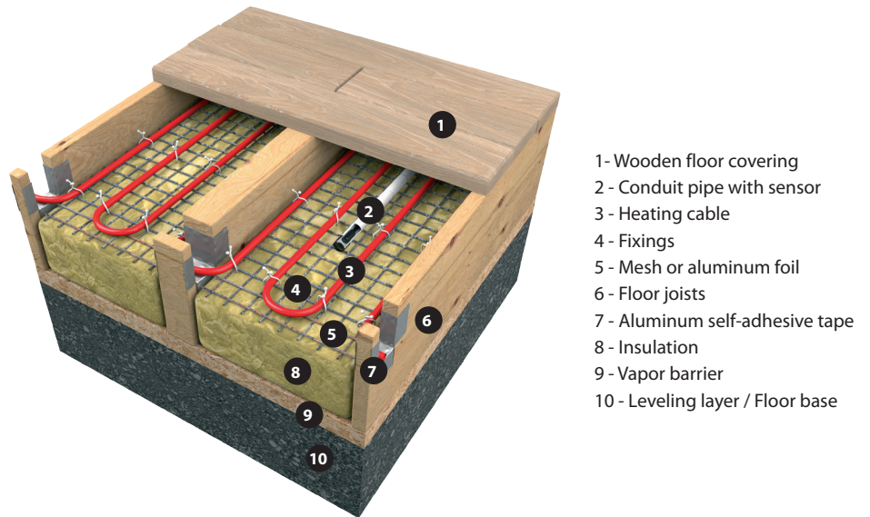
Fig. 13. Wooden floor on joists
