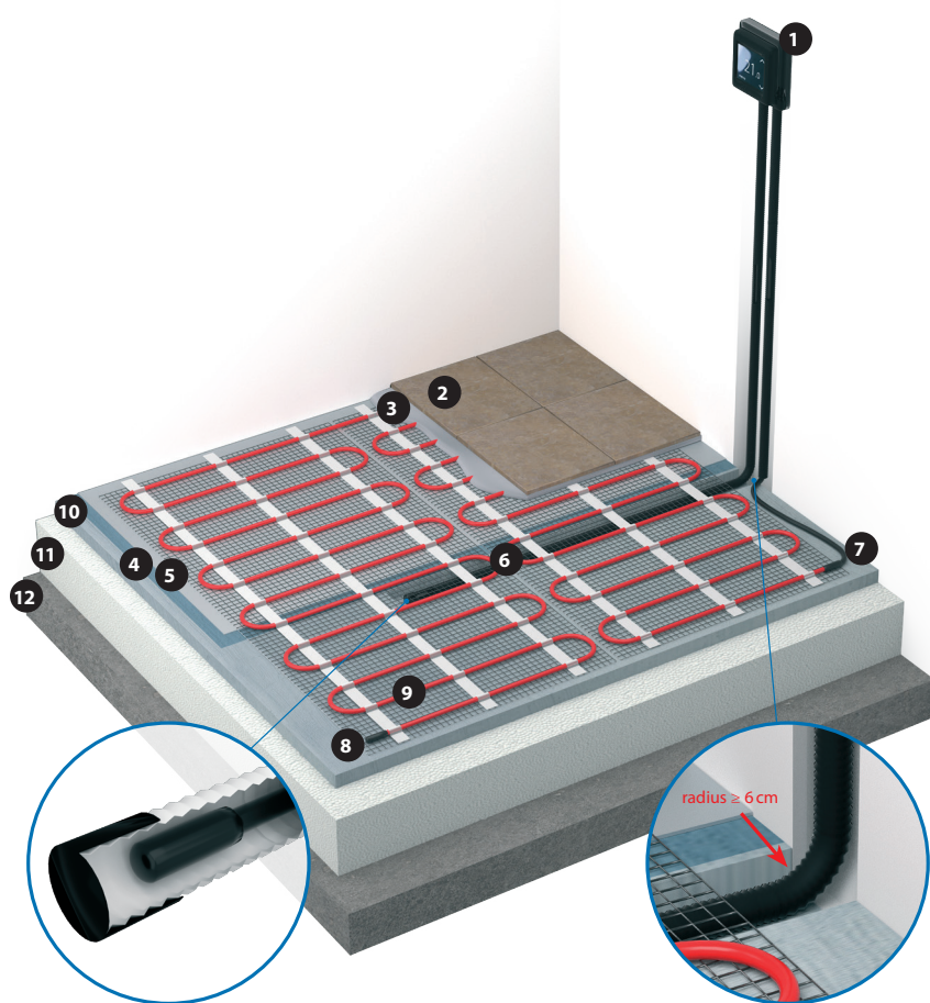
Fig. 6. Thin floor construction with twin conductor thin heating mat
