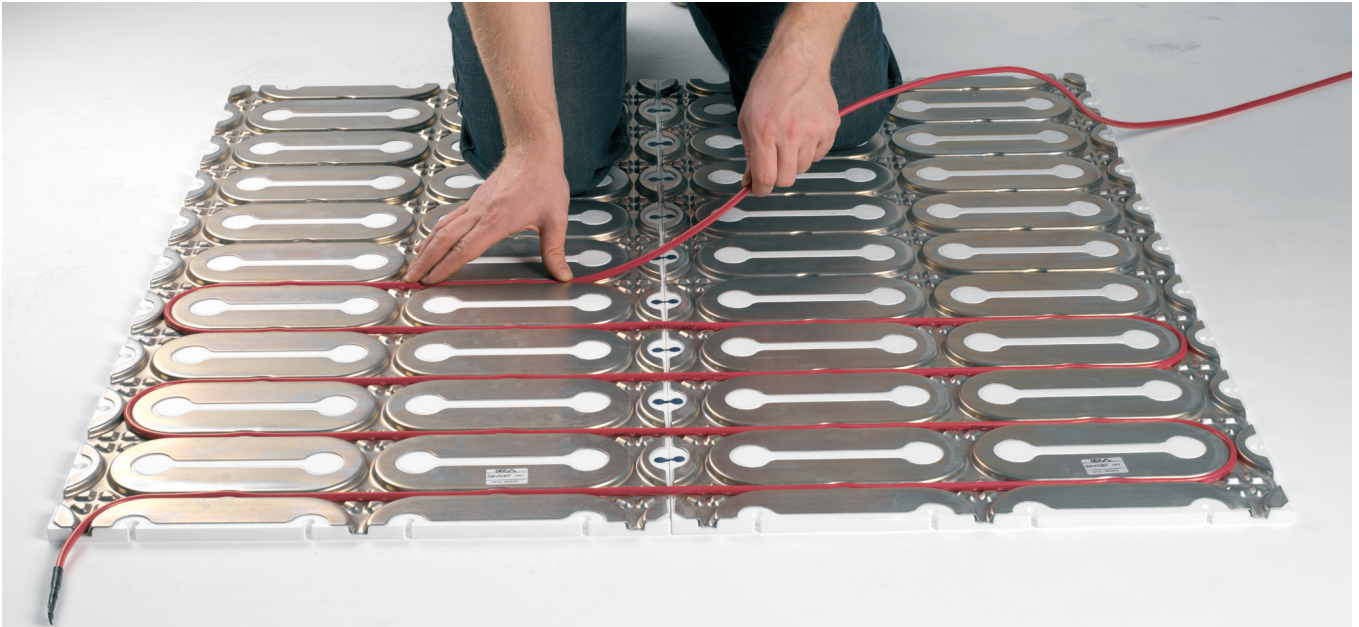
Fig. 20. Mounting method for heating cable into DEVIcell™
