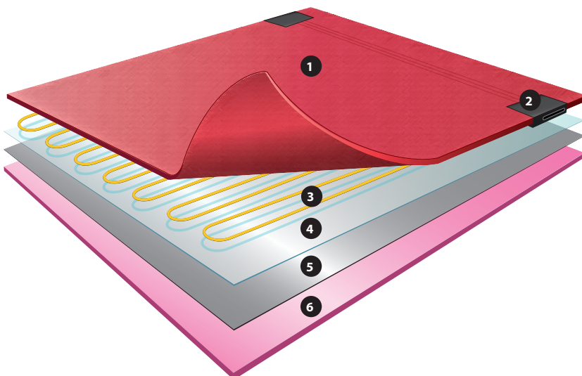
Fig. 15. DEVIDry™ heating element construction
