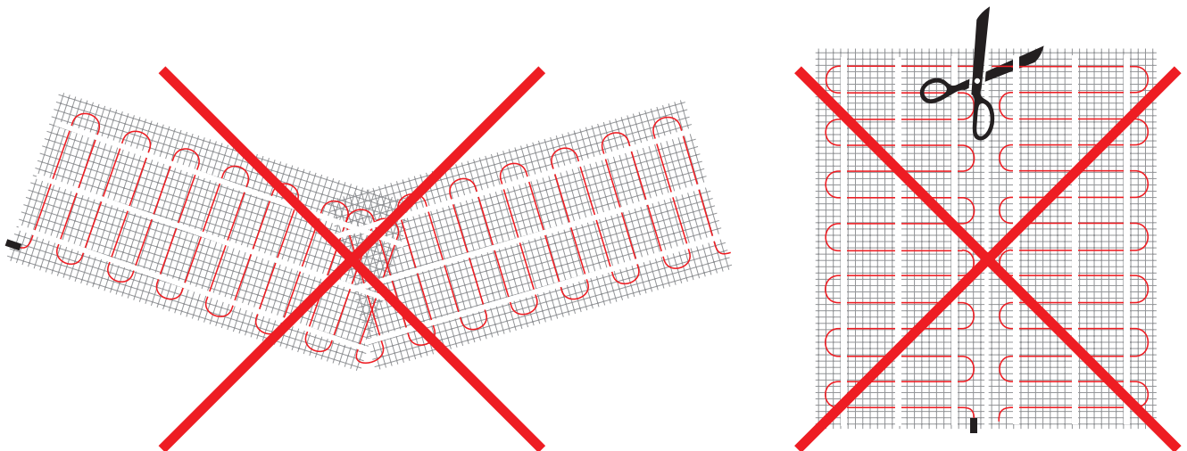
Fig. 10. Never cross or cut cable on the heating mat.
