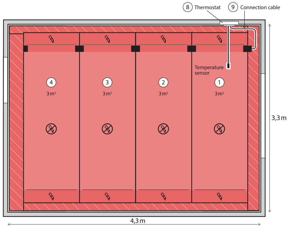
Fig. 18. Connectors along top wall and place for thermostat installation (connection to heating elements) at top-right corner of the room.
